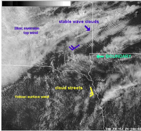
Figure 4. Example slide from the RSO 3 teletraining session showing a visible satellite image with different cloud types and air masses labeled.
