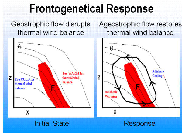
Figure 7. Cross-section showing the ageostrophic response to frontogenesis.
