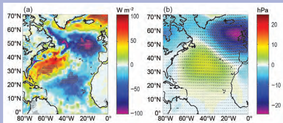
FIG. SB3.2. (a) ERA-Interim net heat flux anomaly (colored field, blue shows increased net ocean heat loss in \text{W m}^{-2} ) for Jan–Feb 2014 relative to the 1972–2012 climatological mean for these months. Stippling indicates regions in which the net heat flux anomaly in Jan–Feb 2014 was the strongest in this two month interval since 1979. (b) Corresponding OAFlex wind field anomaly and ERA-Interim sea level pressure anomaly.
