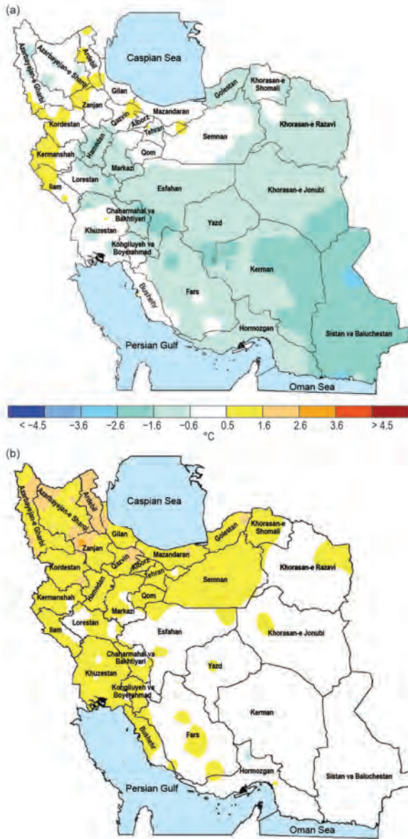
FIG. 7.41. Seasonal mean surface temperature anomalies ( ^{\circ}\text{C} ) in (a) winter (Dec–Feb) 2013/14, and (b) spring (Mar–May) 2014. (Source: I. R. of Iranian Meteorological Organization & National Center for Drought and Disaster Risk Management.)
