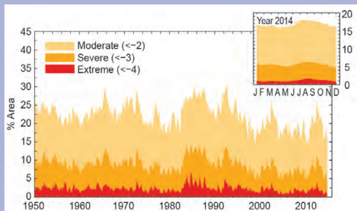
FIG. SB2.3. Percentage of global land area with scPDSI indicating moderate (<math>< -2</math>), severe (<math>< -3</math>) and extreme (<math>< -4</math>) drought for each month for 1950–2014. Inset: each month of 2014.
