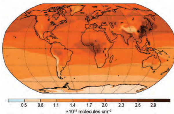
FIG. 2.50. Monitoring Atmospheric Composition and Climate (MACC) reanalysis average total column CO for the period 2003–14 ( \times 10^{18} molecules \text{cm}^{-2} ).
