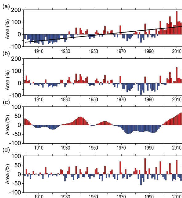
FIG. 4.38. The AWP index from 1900 to 2014. The AWP area index (% deviations from normal) is calculated as the anomalies of the area of SST warmer than 28.5^{\circ}\text{C} divided by the climatological Jun–Nov AWP area. Shown are the (a) total, (b) detrended (removing the linear trend), (c) multidecadal, and (d) interannual area anomalies. The multidecadal variability is obtained by performing a 7-year running mean to the detrended AWP index. The interannual variability is calculated by subtracting the multidecadal variability from the detrended AWP index. The black straight line in (a) is the linear trend fitted to the total area anomaly. The extended reconstructed SST dataset is used.
