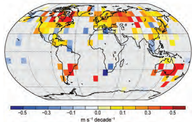
FIG. 2.33. Trends (color scale, \text{m s}^{-1} \text{decade}^{-1} ) of homogenized U-wind component for period 1958–2010 at the 300-hPa level as described in Ramella-Pralungo and Haimberger (2014). Note that positive (negative) changes in the zonal wind speed imply an increase in westerlies (easterlies). 10^{\circ} \times 10^{\circ} grid boxes are only filled if at least one balloon wind record with at least 45 years of data was present.
