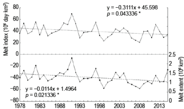
FIG. 6.7. Upper panel: Melt index ( 10^6 day·km ^2 ) from 1978/79 to 2015/16, showing a negative trend (311 100 day·km ^2 yr ^{-1} , p < 0.05 ). Lower panel: Melt extent ( 10^6 km ^2 ) from 1978/79 to 2015/16, showing a negative trend (11 400 km ^2 yr ^{-1} , p < 0.05 ). Year on the x-axis corresponds to the start of the austral summer melt season, e.g., 2008 corresponds to summer 2008/09.
