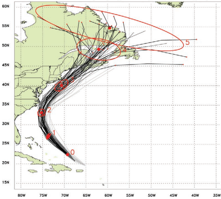
FIG. 5. Lagged ensemble track forecasts for Hurricane Earl (2010) from the GFS/EnKF (see Hamill et al. 2011a). Light grey lines denote track forecasts initialized at 0000 UTC 31 Aug 2010. Darker grey lines denote track forecasts initialized at 1200 UTC 31 Aug 2010. Black lines denote track forecasts initialized at 0000 UTC 1 Sep 2010. Red dots denote positions of ensemble members, with the large red dot the position of the ensemble-mean member. The ellipse is from a fitted bivariate normal distribution, with the contour enclosing 90% of the fitted probability (ibid.). Numbers indicate the forecast lead in days corresponding to the 1 Sep forecast.
