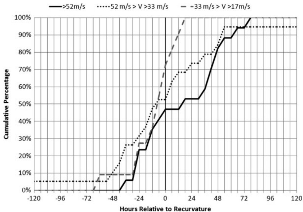
Figure 7. The cumulative distribution of timing of maximum intensity with respect to the point of recurvature for all TCs whose maximum intensities reach tropical storm ( 17 \text{ m s}^{-1} < V_{\text{max}} < 33 \text{ m s}^{-1} ) hurricane ( 33 \text{ m s}^{-1} < V_{\text{max}} < 52 \text{ m s}^{-1} ) and major hurricane ( V_{\text{max}} > 52 \text{ m s}^{-1} ) strength in the South Pacific Ocean (135°E–135°W).
