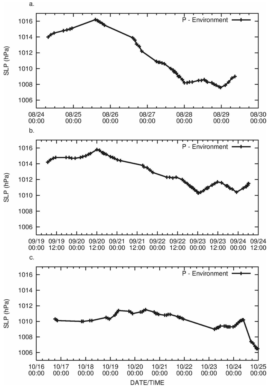
FIG. 2. The time series of environmental pressure ( P - \text{environment} ) for Hurricanes (a) Katrina, (b) Rita, and (c) Wilma. Environmental pressure is defined in KZ07 as the average value in an annulus between 800 and 1000 km from the center of a tropical cyclone.
