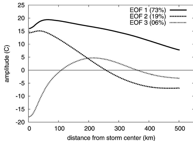
FIG. 2. Leading modes of variability (EOFs) of the 6-hourly mean azimuthally averaged profiles of IR BT. The variance explained by each EOF is shown in parentheses.
