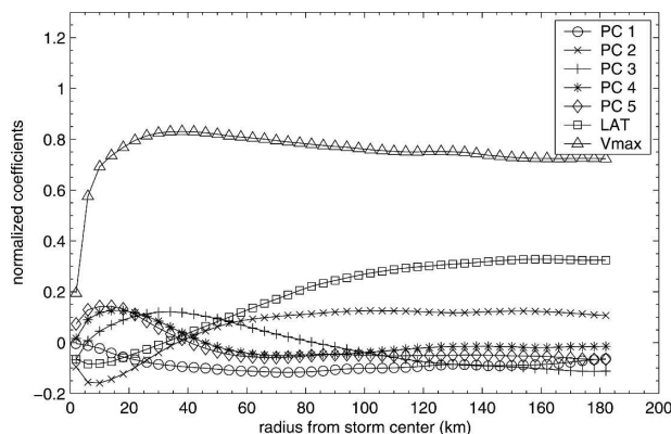
FIG. 4. Normalized coefficients for the SFPCA-regression algorithm at each radius.
