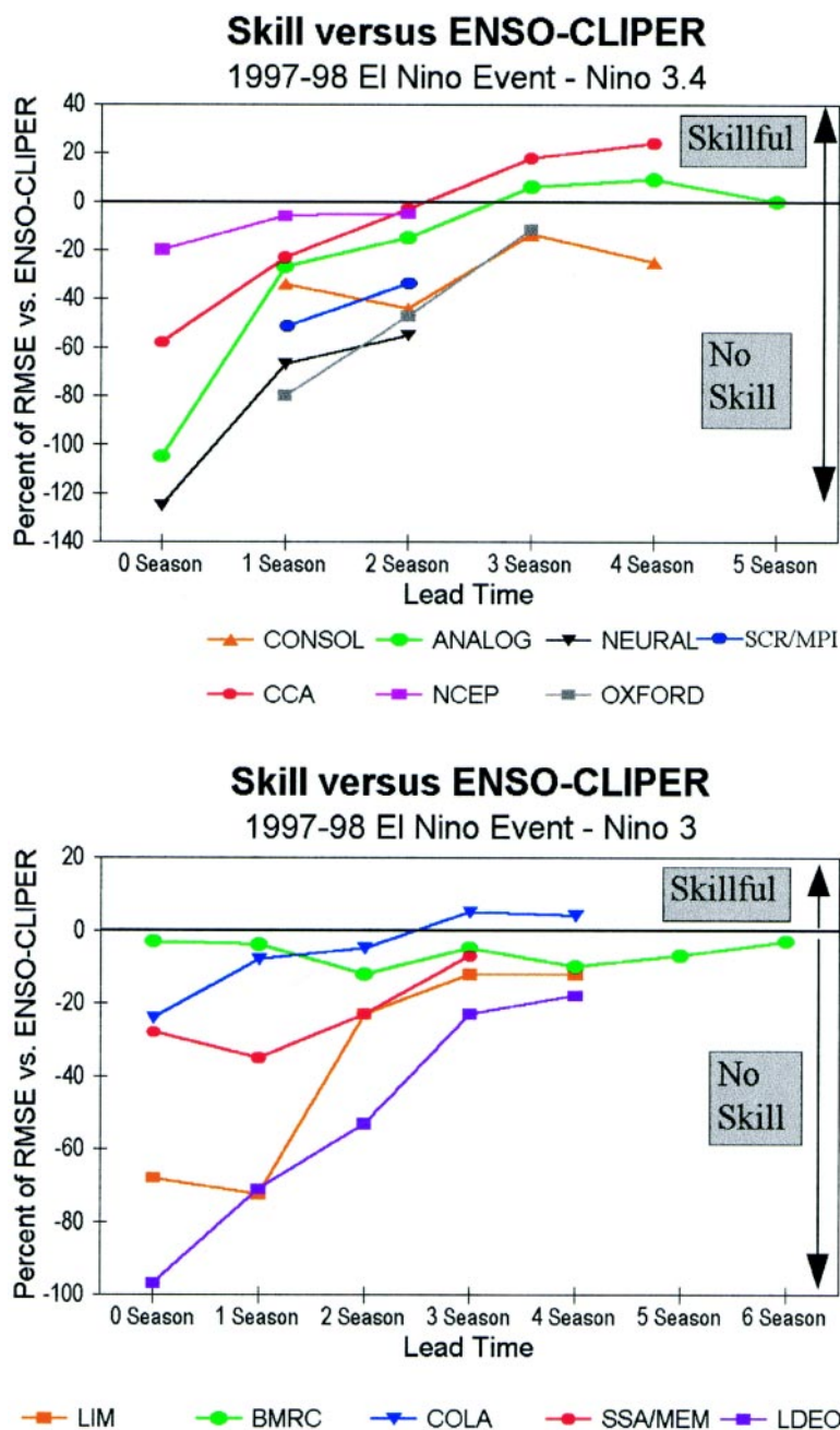
FIG. 3. Skill of various ENSO forecasting methodologies for the 1997–98 El Niño event. Error values for lead times ranging from zero to six seasons in advance are expressed as a percentage of the rmse relative to ENSO–CLIPER. Negative values indicate a forecast performance worse than ENSO–CLIPER and thus no skill. Positive values are improvements over ENSO–CLIPER and thus are “skillful” predictions. Error values are shown for forecasts of (top) Niño-3.4 and (bottom) Niño-3 SST anomalies.
