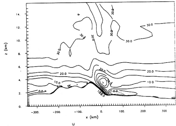
Figure 4. Horizontal wind u -component at 2300 LST. Contour interval is 5 \text{ ms}^{-1} .
