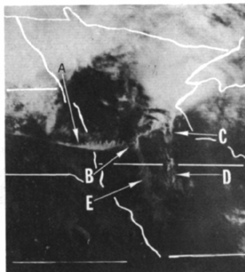
FIG. 5c. GOES-2, 1 km visible imagery, 29 June 1975, 1545 GMT.
