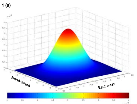
Figure 1(a): This figure represents the normalized probability density function for a GOES-R ABI pixel at 3.9 μm over Kansas representing the point spread function (psf). The nominal pixel size is approximately 2.4 km (East West) X 3.2 km (North-South) while the total area for the psf is 4.8 km X 6.4 km and covers over 99.5% of a bivariate normal pdf. The core area is seen to contain 73% of the total pixel information.
