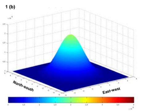
Figure 1(b): This figure represents the normalized probability density function for a GOES-R ABI pixel at 10.35 μm over Kansas representing the point spread function (psf). The nominal pixel size is approximately 2.4 km (East West) X 3.2 km (North-South) while the total area for the psf is 7.2 km X 9.6 km and covers over 99.5% of a bivariate normal pdf. The core area is seen to contain 53% of the total information.
