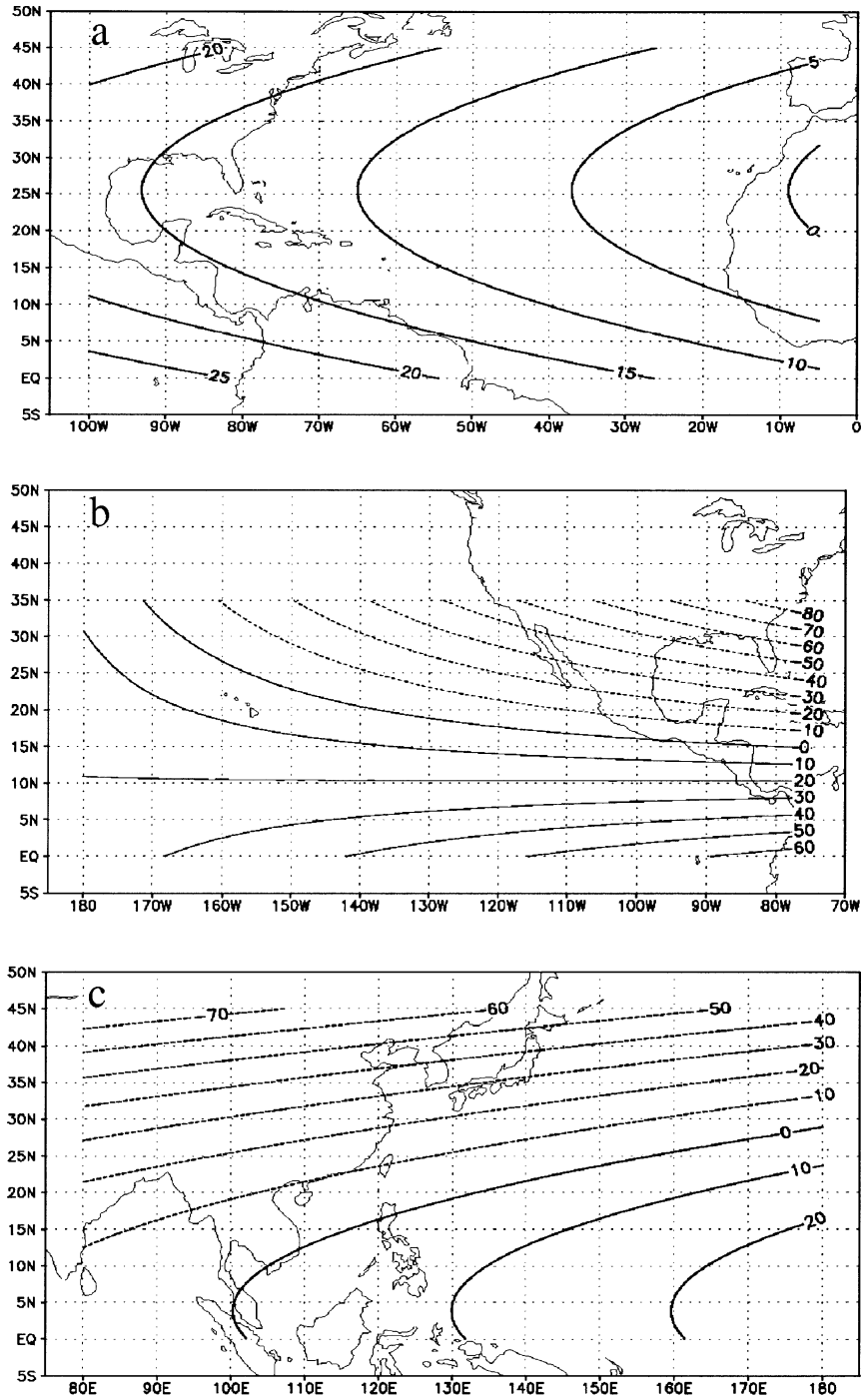
FIG. 3. Examples of the resulting spatial distribution of DELV (kt) calculated from the cross-product terms containing LAT and LON in the 48-h forecasts in the (a) North Atlantic, (b) eastern North Pacific, and (c) western North Pacific tropical cyclone basins. To calculate these distributions, the yearday = 250 (7 Sep), VMAX = 50 kt, DVMAX = 0 kt, U = 10 kt, and V = 2 kt. The contour intervals are 5 kt in the North Atlantic and 10 kt in the other basins.
