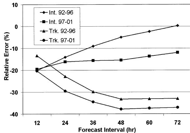
FIG. 1. Relative error of the official NHC track (Trk.) and intensity (Int.) forecasts for 1992–96 and 1997–2001. The zero line represents a CLIPER-based control forecast, so that negative relative errors represent skillful forecasts.
