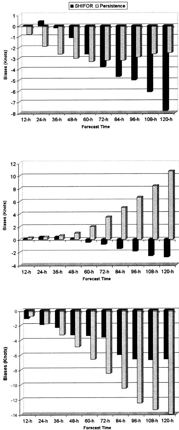
FIG. 6. Intensity forecast biases (kt) from the 5-day SHIFOR and STIFOR models through 120 h, initialized using operational data for 1997–2000, as compared with a forecast of persistence of initial conditions. Biases from the (top) North Atlantic, (middle) eastern North Pacific, and (bottom) western North Pacific are shown. The number of cases is the same as in Fig. 5.
