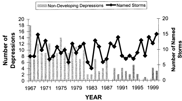
FIG. 2. Time series of the number of annual nondeveloping depressions and named storms in the Atlantic tropical cyclone basin. Note the decrease in numbers of nondeveloping depressions with time while the trend of named storms shows little overall trend.
