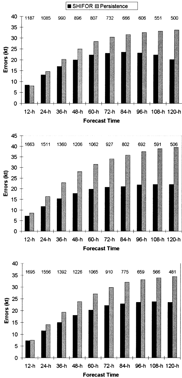
FIG. 5. Mean absolute intensity forecast errors (kt) from the 5-day SHIFOR and STIFOR models through 120 h, initialized using operational data for 1997–2000, as compared with a forecast of persistence of initial conditions. Errors from the (top) North Atlantic, (middle) eastern North Pacific, and (bottom) western North Pacific are shown. The number of cases is shown above the bars in each panel.
