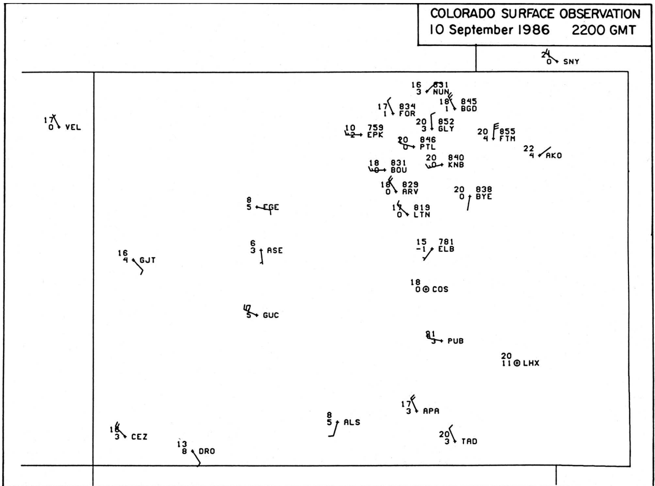
FIG. 6. Surface-weather observations in Colorado on 10 September 1986 at 2200 UTC.
