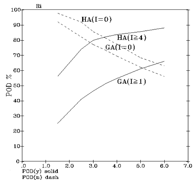
Fig. 1: Verification of the Richardson number ( Ri ) with PIREPs and RUC2 output for the period 1 December 1997 to 10 January 1998. See text for description of figure.
