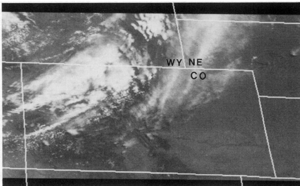
FIG. 5. GOES-7 visible satellite image from 1800 UTC on 3 July 1993 centered over Colorado with portions of surrounding states included.
