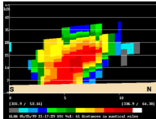
Figure 8. Doppler radar data from the Lubbock, Texas WSR-88D. Image is a vertical cross-section of reflectivity made from the volume scan corresponding to the PPI image shown in Figure 7. North is to the right.
