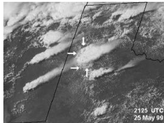
Figure 6. GOES-East visible wavelength image from 2125 UTC on 25 May 1999. Arrows around large storm in west Texas point LTO boundary. Note the new activity forming on the northern side of the storm (northernmost arrow)
