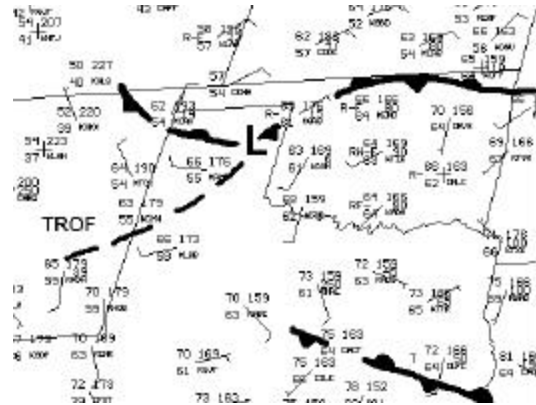
Figure 2. Surface analysis for 1500 UTC on 25 May 1999. Observations in English units, plotting convention is U.S. standard. Surface features from NCEP analysis.
