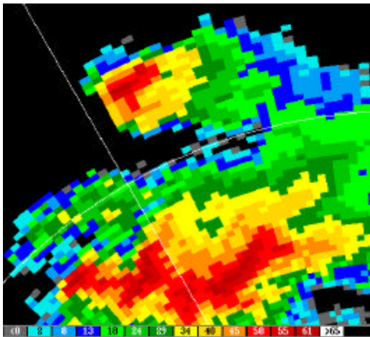
Figure 7. Doppler radar reflectivity data from the Lubbock, Texas WSR-88D. Image shows reflectivity (in dBz) from a 2.4^\circ elevation, PPI scan taken at 2117 UTC on 25 May 1999.
