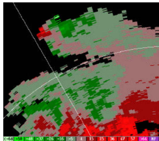
Figure 9. Doppler radar velocity data corresponding to the reflectivity scan shown in Figure 7. Image shows velocities (in kt) toward the radar in grays and green, velocities away from the radar in shades of red.
