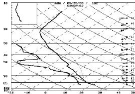
Figure 3. Plot of data from a special radiosonde released at Amarillo, Texas at 1800 UTC on 25 May 1999 on a Skew-T/Log P diagram. Wind speeds are in knots.
