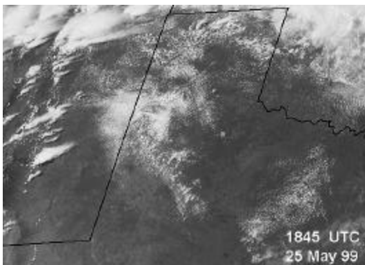
Figure 5. GOES-East visible wavelength image taken at 1845 UTC on 25 May 1999. The northwest-southeast oriented line of enhanced cloudiness near center of the image is the convergence line referred to in the text.
