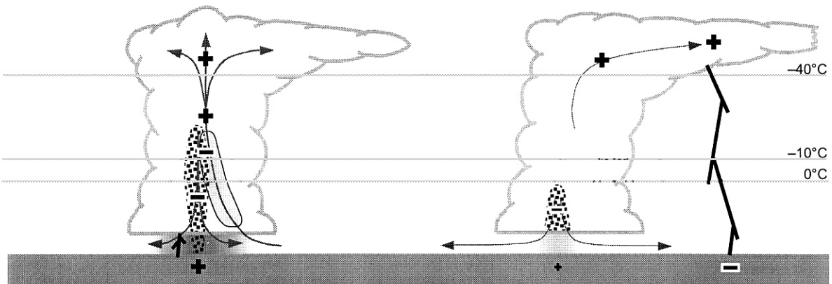
Fig. 1c – Mature Cumulonimbus
