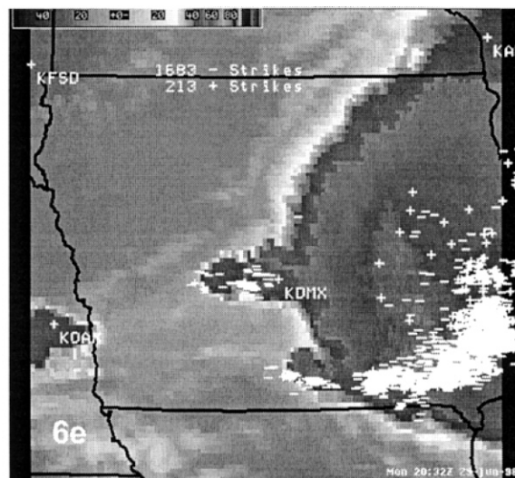
Fig. 6. Satellite and lightning data from 17:32–20:32 UTC on 29 June 1998 over Des Moines, Iowa. Infrared satellite imagery from GOES-8 (Ch. 4; 10.7 \mu\text{m} ) and 15-minute CG lightning data. Satellite imagery is displayed as infrared blackbody temperature. The arrow in the Fig. 6a provides reference to the -40^{\circ}\text{C} contour. Satellite scan time is listed in the lower right corner. Counts of - CGs and + CGs are listed. State boundaries and locations of WSR-88D radar are shown.
