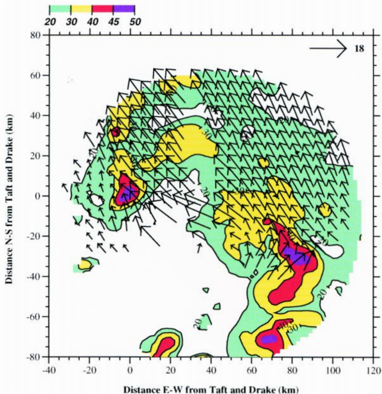
a. 28 JULY 1997, 2110 MDT: dBZ/H-WIND (Z=1 KM)
