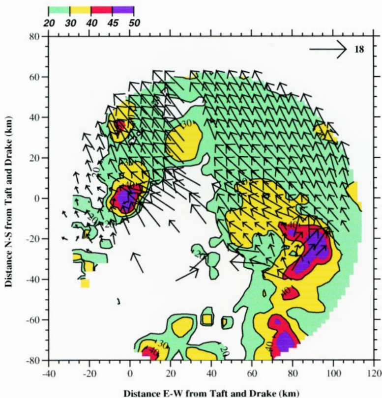
b. 28 JULY 1997, 2130 MDT: dBZ/H-WIND (Z=1 KM)
