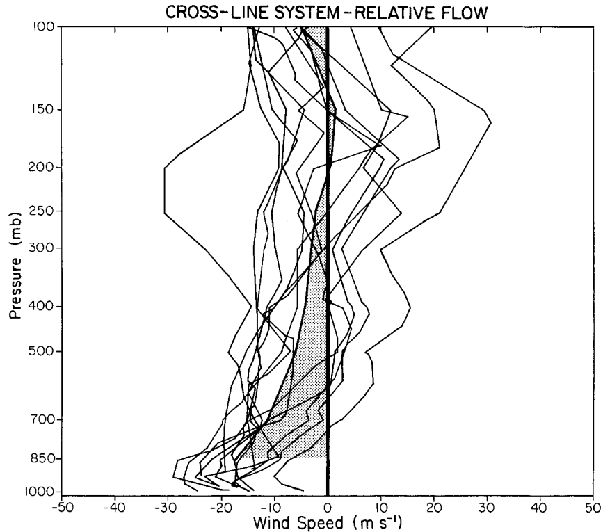
FIG. 14. Same as Fig. 13 except for cross-line, system-relative flows. Positive speed is rear to front.
