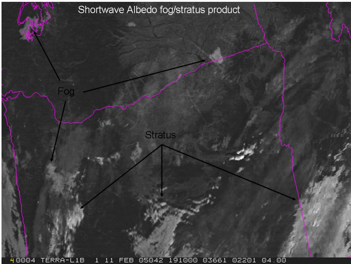
Figure 1a: Shortwave Albedo Product showing patches of fog and stratus in southern Washington and Oregon at 1910 UTC (daytime) on 11 February 2005. Fog and stratus are white/light, whereas ice clouds and most land surfaces are dark.
