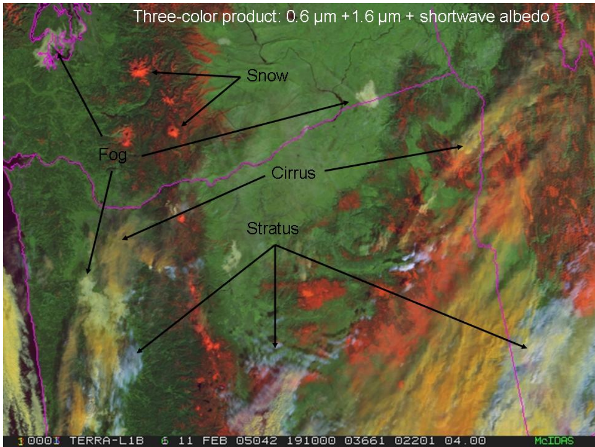
Figure 1c: New Fog/Stratus Three-Color Product that better discriminates clouds from land, and between different levels and types of clouds, for the same scene as in Figure 1a and 1b. Snow is orange/red; high-level cirrus/ice clouds are yellow/orange; low-level stratus/water clouds have a blue tint; and fog (on the ground) is whiter than stratus clouds that are off the ground. Most land surfaces are green, the color discrimination of different land types being sacrificed for cloud level and type discrimination.
