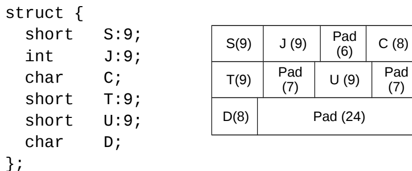
Figure 17-4. Storage unit sharing and alignment padding, sizeof is 12
