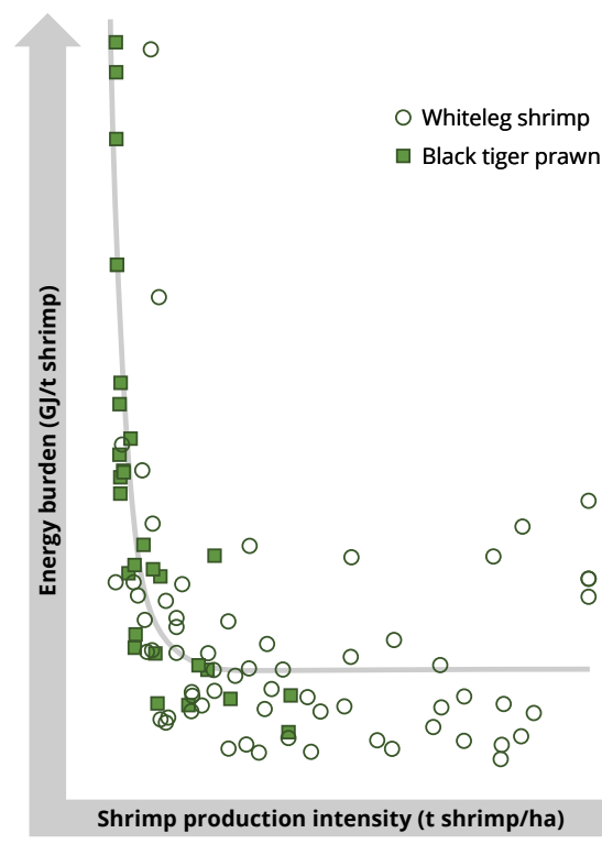
Figure 10. Combined energy use (operational, construction and embodied) for shrimp production as a function of farm intensity
