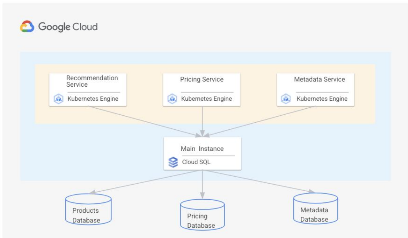
Microservices architecture
