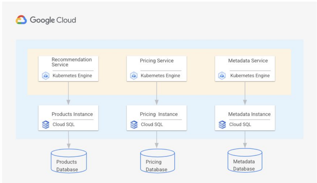
Microservices architecture
