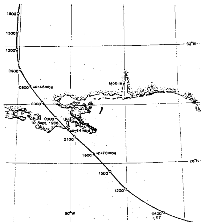
Figure 21. Meteorological input parameters for Hurricane Betsy, 1965.
