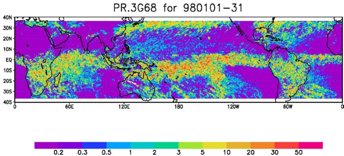
Fig. 6. Global precipitation distribution of the TRMM PR Rainsurf for (a) January, (b) April, (c) July, and (d) October 1998.
