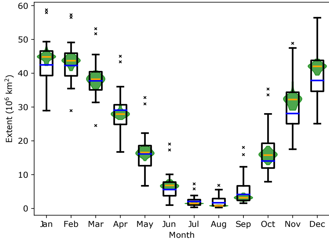
(b) CMIP6 NH snow extent (1981–2014)
