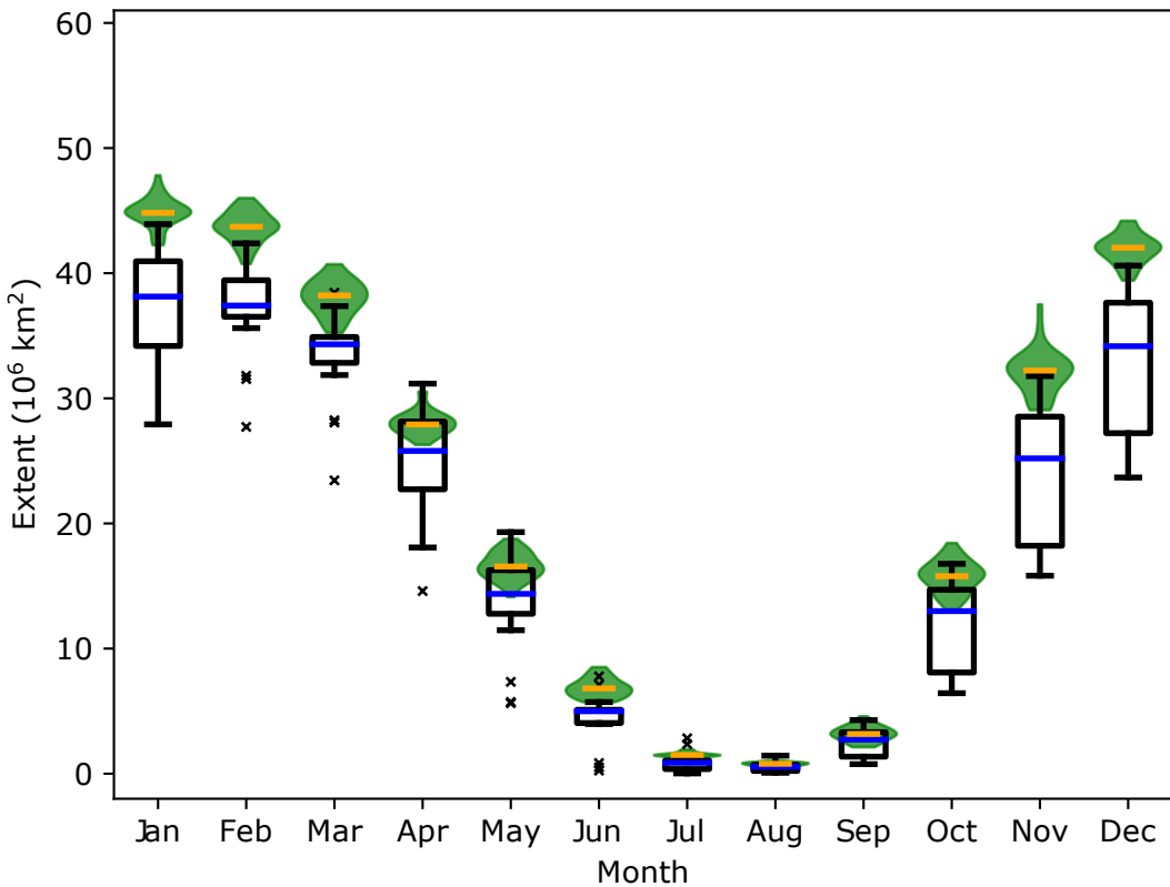
(a) CMIP5 NH snow extent (1981–2014)
