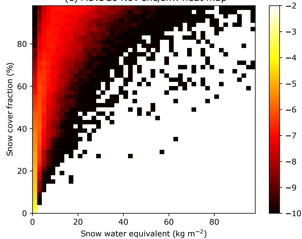
(c) MIROC6 Nov snc/snw heat map
