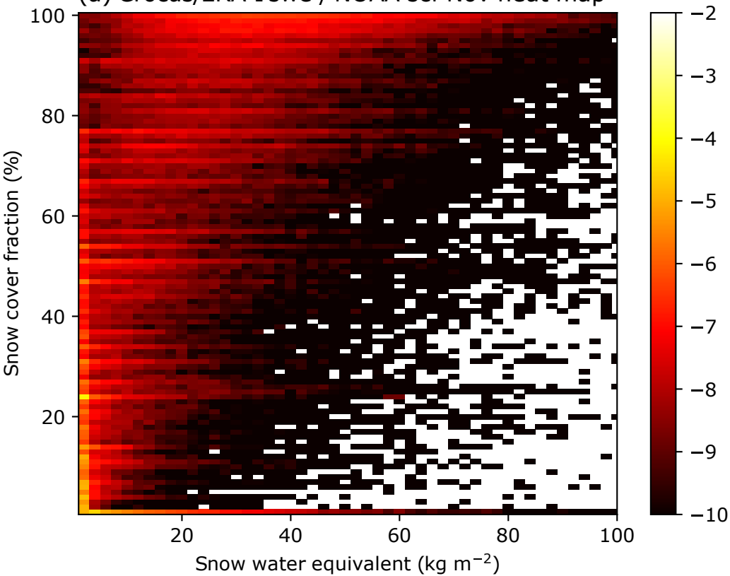
(a) Crocus/ERA-I swe / NOAA scf Nov heat map
