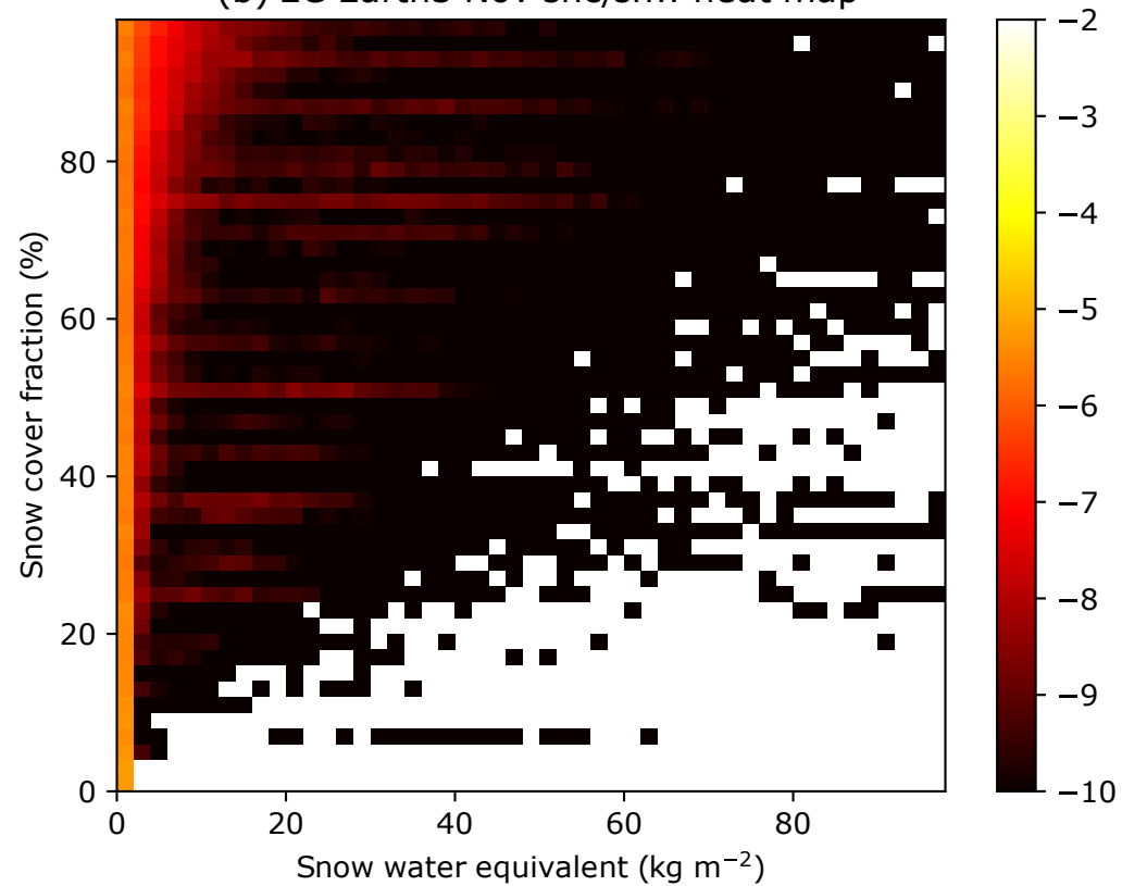
(b) EC-Earth3 Nov snc/snw heat map
