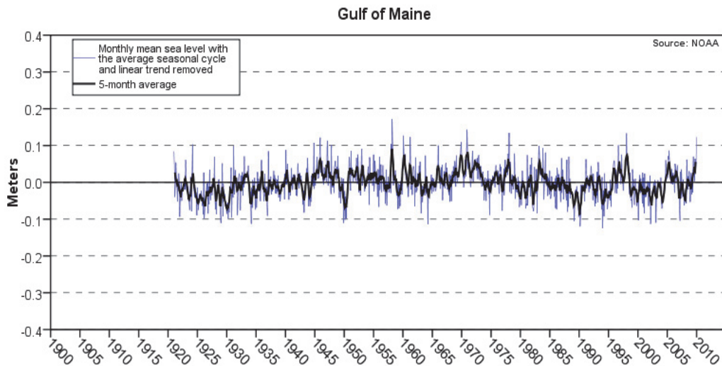
Figure 2. The regional oceanographic residual using an average of the data from Eastport, ME to Boston, MA
