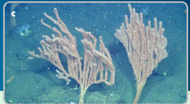
ROV Hercules seafloor photos of: (a) rock fish in Quinault Canyon, Olympic Coast National Marine Sanctuary, (b) glass sponge in Grays Reef, and (c) bamboo coral found on accretionary ridges.
