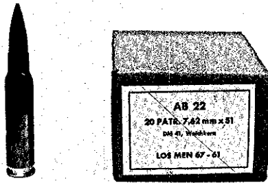
Patrone 7,62 mm × 51 DM41, Weichkern
