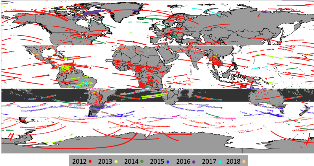
Figure 3 (continued): Annual global distribution of spurious VNP14 fire pixels associated with poorly-calibrated SDR input data acquired between Jan 2012- Jun 2018. Map shows data from 187 separate granules.
