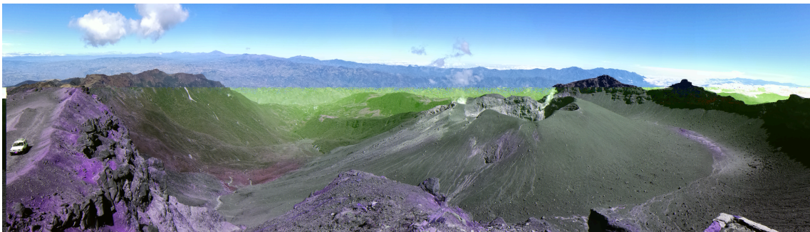
Galeras Volcanic Complex. Picture by the Volcano Geology Team, Servicio Geológico Colombiano
