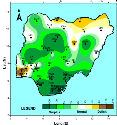
Fig.5: 1 st DEKAD OF SEPTEMBER SOIL MOISTURE INDEX (SMI)
