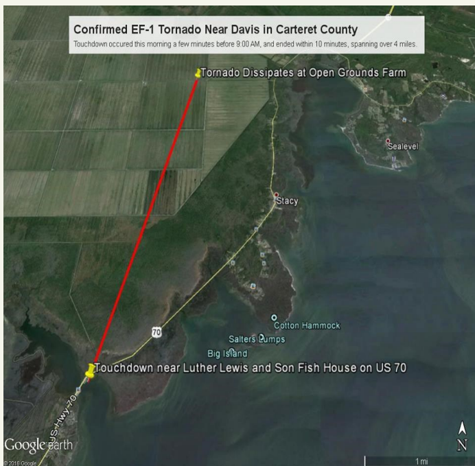
Path of EF-1 tornado in Carteret County, February 16, 2016.
