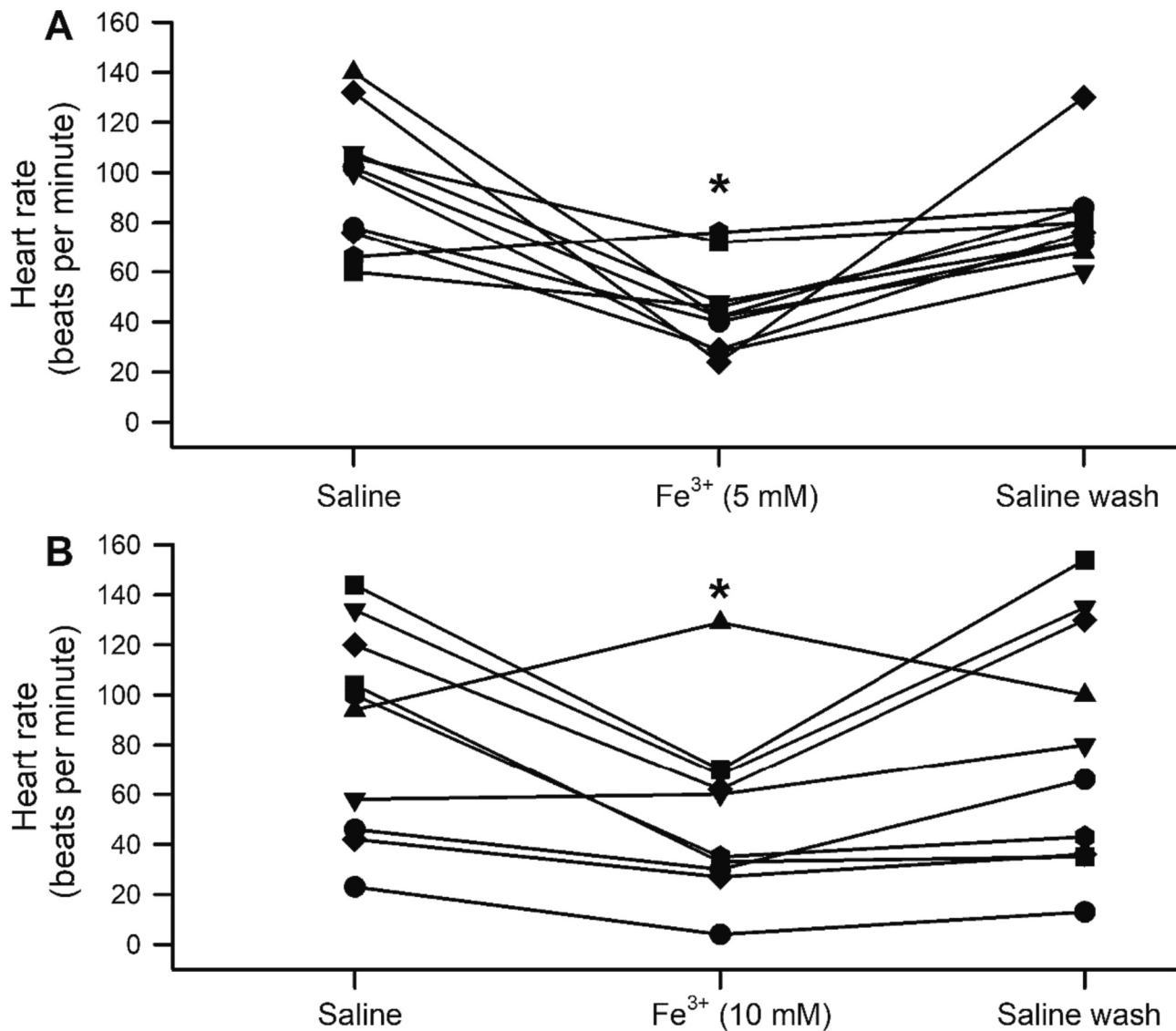
Fig. 7. The effect of acute exposure to iron on the in situ 3rd instar larval heart. The in situ larval heart tube was exposed to ferric ammonium citrate at (A) 5 mM or (B) 10 mM followed by exchanging the bathing solution to fresh saline without ferric ammonium citrate. The rate was determined for 1 min during exposure to ferric ammonium citrate and after 2 bath exchanges to fresh saline. A paired t -test from initial saline to ferric ammonium citrate with normality test (Shapiro-Wilk) revealed significant differences for both concentrations (*, p < 0.05 ) without differences in the responses between concentrations. n = 10 for each concentration.
