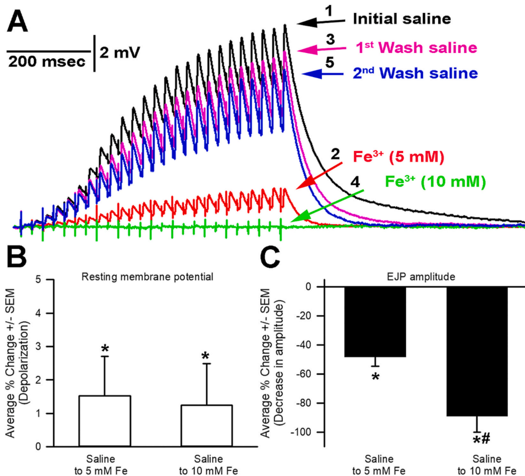
Fig. 11. The effect of ferric ammonium citrate on membrane potential and evoked excitatory junction potentials (EJPs) at the neuromuscular junction of the opener muscle in the walking leg of crayfish. (A) The motor nerve was stimulated at a rate of 40 Hz with 25 pulses. Ferric ammonium citrate (5 mM) rapidly depolarized the depressed evoked synaptic transmission. With the bath exchange back to fresh saline the EJP amplitudes were revived. Upon exposure a subsequent higher concentration of ferric ammonium citrate (10 mM) evoked synaptic transmission was depressed to a greater extent than 5 mM. (B) The exposure to 5 mM and 10 mM ferric ammonium citrate did not significantly depolarize the membrane potential (paired t -test from initial saline to ferric ammonium citrate with normality test by Shapiro-Wilk; p > 0.05 ; N = 6 ). However, a Sign test did illustrate a consistent significant depolarization upon exposure to 5 or 10 mM but the changes were only 1 to 5 mV ( P < 0.05 ; Wilcoxon rank sum test; *). In normalizing the variation in the initial values with determining a mean percent change illustrated small changes. (C) The depression in the EJP amplitude was significant for both the 5 and 10 mM ( p < 0.05 for both 5 and 10 mM before and during exposure and between 5 and 10 mM; non-parametric Wilcoxon rank sum test; n = 6 ; *). The mean percent change was greater for 10 mM than 5 mM (non-paired t -test; p < 0.05 ; #).
