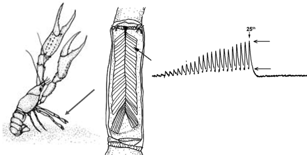
Fig. 2. The walking leg of the crayfish houses the opener muscle used to address the effects of ferric ammonium citrate on synaptic transmission in a crustacean model. Schematic of opener muscle as seen from a ventral view. Excitatory junction potentials were obtained from the distal muscle fibers. The excitatory motor neuron was stimulated at 40 Hz for 25 stimuli. The amplitude of the 25th EJP in the train was used for quantitative purposes.
