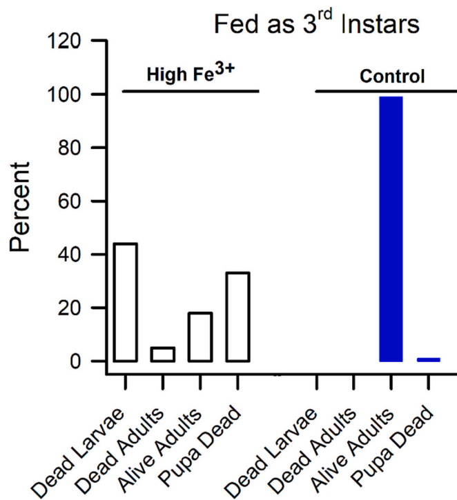
Fig. 4. The effect of dietary Fe 3+ (ferric ammonium citrate) on survival of Drosophila larval from 3rd instar to adulthood. The larvae were fed Fe 3+ starting from the 3rd instar 5 mM (High) and monitored through development to pupation and adulthood. The Fe 3+ was mixed with standard cornmeal food. The larvae and pupa as well as adults had an increase in death rate compared to control (chi-square post-hoc analysis). 10 larvae in 10 different vials for each condition were used; thus, n = 100 for each condition.
