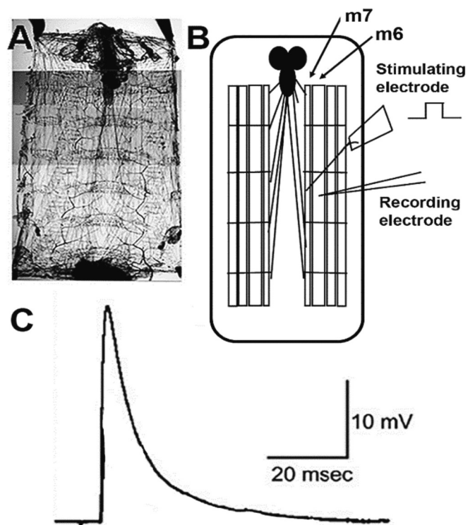
Fig. 1. The larval Drosophila preparation for recording synaptic responses at the neuromuscular junctions. (A) A 3rd instar larvae pinned open and (B) schematically illustrated where a segmental nerve is stimulated to evoke (C) EJPs in m6 muscle fibers.
