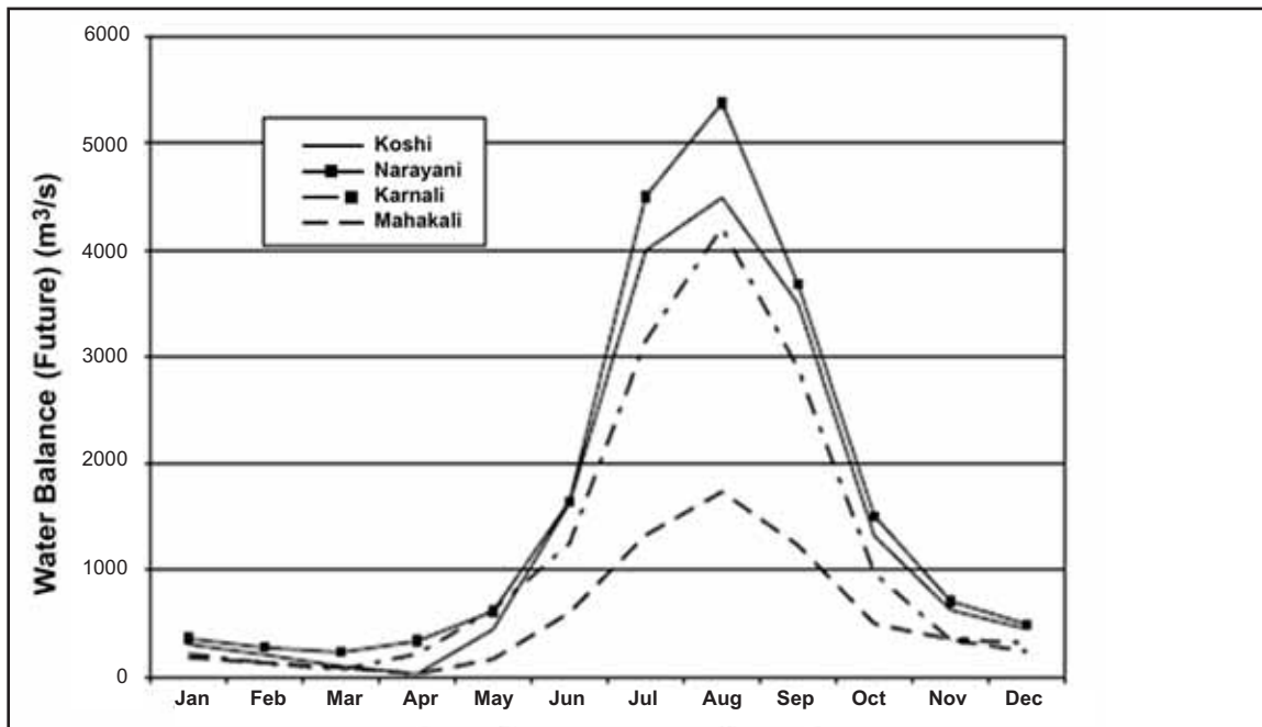
Figure 4: Water balance in the major basins
