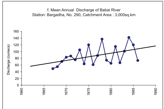
Figure 10: Trend of annual discharge of the major rivers of Nepal (Shrestha et al., 2003)
