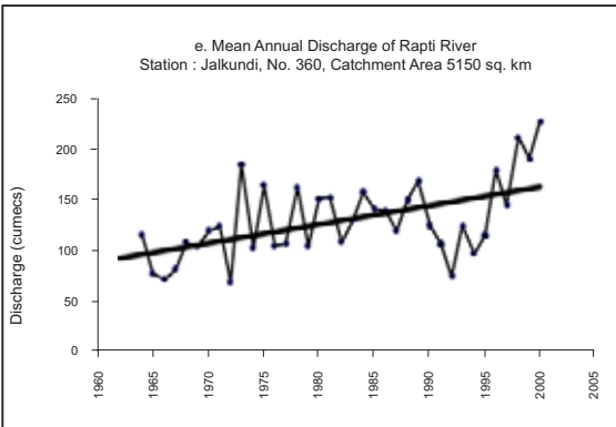
Figure 10: Trend of annual discharge of the major rivers of Nepal (Shrestha et al., 2003)
