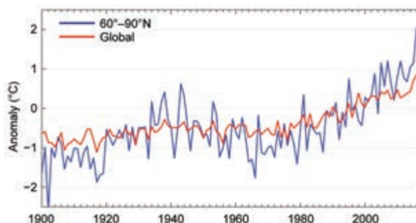
FIG. 5.1. Arctic (land stations north of 60°N) and global mean annual land surface air temperature (SAT) anomalies (°C, 1981–2010 base period) for 1900–2017. Note that there were few stations in the Arctic, particularly in northern Canada, before 1940. (Source: CRUTEM4 dataset.)
