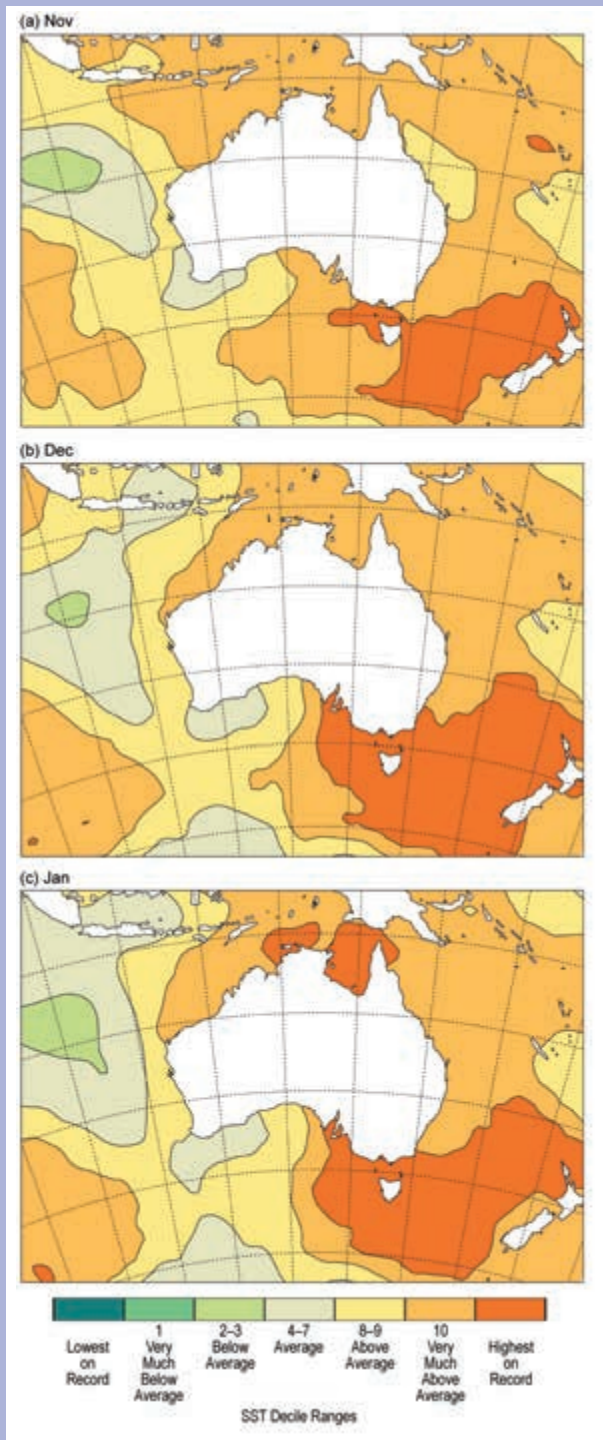
FIG. SB7.7. SST deciles for (a) Nov and (b) Dec 2017 and (c) Jan 2018, based on the 1900–2017 distribution using the NOAA ERSST v5 dataset. (Source: Australia Bureau of Meteorology.)
