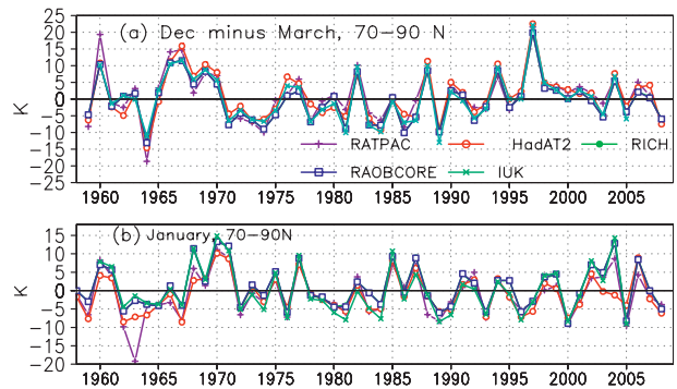
FIG. 6. (a) Time series of difference between temperature anomalies for December and those for March at 50 mb for 70°–90°N for five radiosonde datasets. (b) Time series of temperature anomalies at 50 mb from 70° to 90°N for January for five radiosonde datasets.
