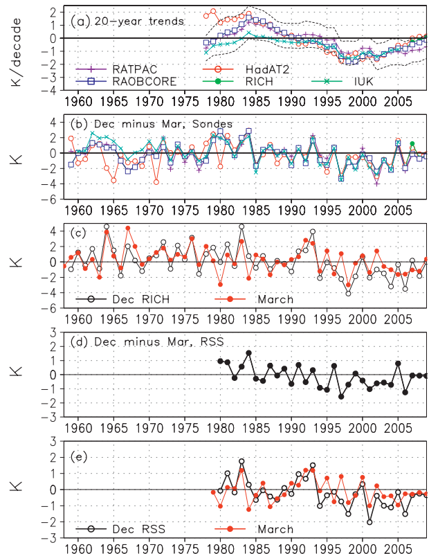
FIG. 4. (a) Temperature trend for December minus trend for the following March at 50 mb in the deep tropics, for sliding 20-yr time periods, plotted by the last year of the time period. Dotted lines denote the 95% confidence interval of the RATPAC trends. (b) Time series of difference between temperature anomalies for December and those for March at 50 mb for 10^{\circ}\text{N} – 10^{\circ}\text{S} for five radiosonde datasets. (c) Temperature anomalies in RICH radiosonde data at 50 mb between 10^{\circ}\text{N} and 10^{\circ}\text{S} , for December and March. (d) Temperature for December minus temperature for March for MSU lower stratosphere temperature between 10^{\circ}\text{N} and 10^{\circ}\text{S} using RSS data. (e) As in Fig. 4c, but for RSS lower stratospheric temperatures. For all panels, data are plotted according to the year in which March occurs.
