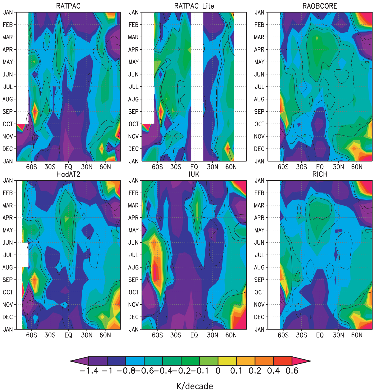
FIG. 2. Trends for 1979–2009 (except for IUK, which is 1979–2005) at 50 mb for 10^{\circ} zonal mean radiosonde temperatures, calculated for individual months, in \text{K decade}^{-1} . Solid black lines enclose the areas where trends are significant at the 95% confidence level; dashed lines indicate areas with 99% significance.
