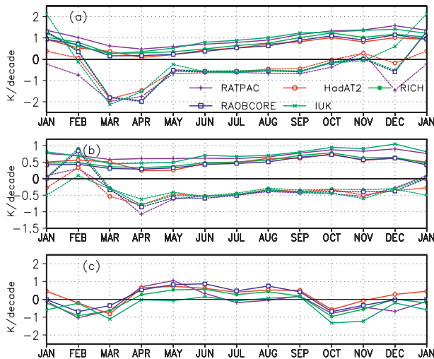
FIG. 5. (a) Trends for 1979–2009 at 50 mb from 10°N to 10°S (solid lines), multiplied by -1 for comparison, and from 70° to 90°N (dotted lines). (b) As in Fig. 5a, but for 1960–2009. (c) Trends for 1995–2009 for 10°N–10°S in radiosonde data.
