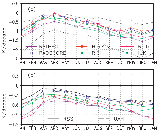
FIG. 3. (a) Trend for 1979–2009 ( K \text{ decade}^{-1} ) at 50 mb, averaged for 10^{\circ}\text{N} – 10^{\circ}\text{S} , calculated by month. Dotted lines represent the limits of the 95% confidence interval for RATPAC. (b) Trends in RSS and UAH MSU lower stratosphere temperature and equivalent temperatures calculated from radiosonde datasets, for 1979–2009, for 10^{\circ}\text{N} – 10^{\circ}\text{S} , by month.
