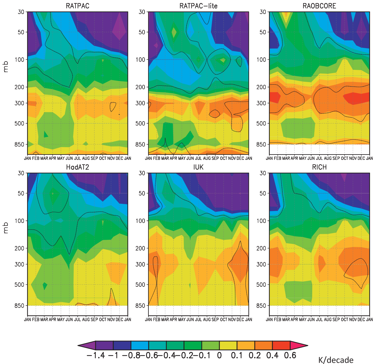
FIG. 1. Trends ( \text{K decade}^{-1} ) in radiosonde temperature data from six datasets, averaged for 10^{\circ}\text{N} – 10^{\circ}\text{S} for 1979–2009 (2005 for IUK), calculated for individual months. Black lines enclose the areas where trends are significant at the 95% confidence level.
