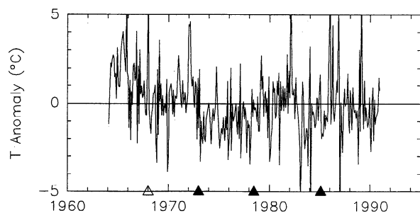
Figure 2. Time series of 50-hPa monthly temperature anomalies at De Bilt, the Netherlands. Open arrow shows date of known change in radiation corrections, while solid arrows show dates of radiosonde type changes, as noted in the text.
