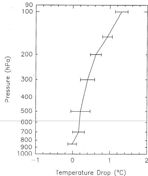
Figure 9. Average and standard deviation, over 13 stations, of the drop in temperature associated with the 1968 lengthening of radiosonde cords in Japan, as a function of pressure.
