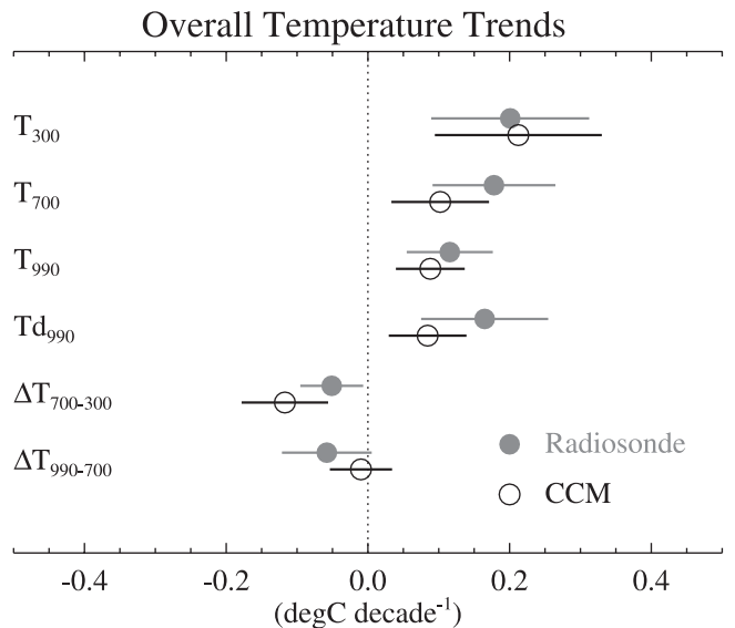
Figure 5. Overall tropical radiosonde (solid circles) and CCM (open circles) trends (in degC decade -1 ) for temperature at 300 hPa ( T_{300} ), temperature at 700 hPa ( T_{700} ), temperature at 990 hPa ( T_{990} ), dew-point temperature ( Td_{990} ), temperature difference 700–300 hPa ( T_{700-300} ), and temperature difference 990–700 hPa ( T_{990-700} ). Trends are indicated by the circle, and the 95% confidence interval is indicated by the horizontal bar.
