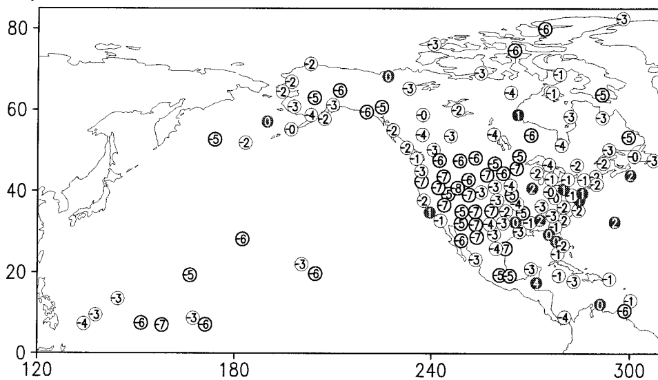
FIG. 3. Spearman correlation coefficients between annual anomalies of temperature and relative humidity at (a) 850 and (b) 700 hPa. The shading and outlining are as in Fig. 1.
