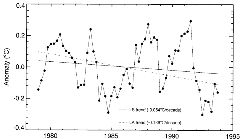
Figure 3. Time series of seasonal-mean lower tropospheric ( 2_{LT} ) temperature anomalies ( ^{\circ}\text{C} ) over 1979–1993 in MSUd. Note that the LS and LA linear fits yield a trend difference of 0.085^{\circ}\text{C}/\text{decade} .
