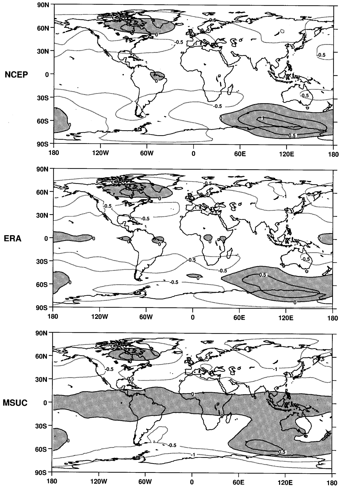
Figure 10. Lower-stratospheric temperature trends over 1979–1993 (in ^{\circ}\text{C}/\text{decade} ) in the NCEP, ERA, and MSUC data. Equivalent channel 4 temperatures from NCEP and ERA were computed with a radiative transfer code. The contour interval is 0.5^{\circ}\text{C} , and areas with positive changes are shaded.
