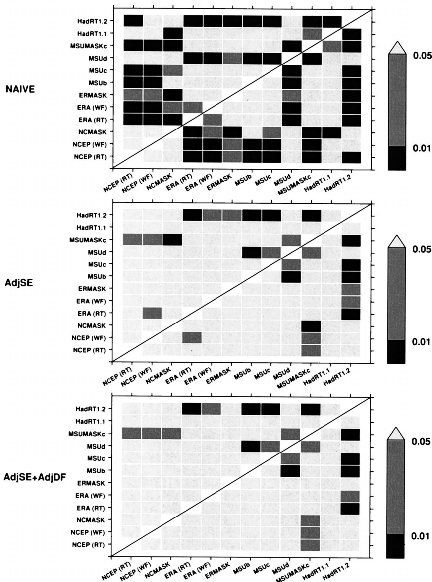
Figure 9. Significance of midtropospheric (channel 2) trend differences between various data sets, as assessed by the “NAIVE,” “AdjSE,” and “AdjSE + AdjDF” approaches (see section 4). All three test the significance of the trend in the difference time series d(t) . Tests involve global-mean seasonal-mean anomaly data spanning the period 1979–1993. Matrices are symmetrical about the diagonal line.
