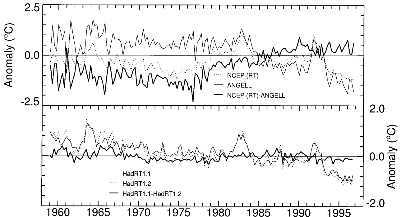
Figure 1. Time series of global-mean seasonal-mean temperature anomalies ( ^{\circ}\text{C} ) in the lower stratosphere. (top) Results for ANGELL's radiosonde-based 50–100 hPa thickness temperatures, the equivalent MSU channel 4 temperatures obtained from the NCEP reanalysis, and the difference between NCEP and ANGELL. (bottom) The equivalent channel 4 time series estimated from the HadRT1.1 and HadRT1.2 radiosonde data, together with their difference time series.
