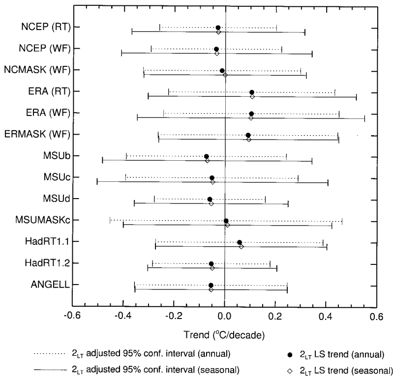
Figure 8. Sensitivity of confidence intervals for 2_{LT} least squares linear trends to sampling interval. Trends and adjusted 95% confidence intervals (see section 5.1) were computed with both seasonal-mean and annual-mean anomaly data spanning the period 1979–1993.
