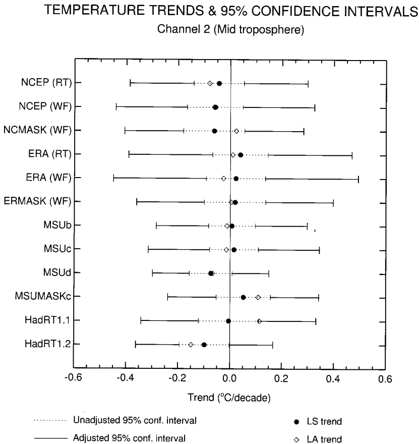
Figure 6. As for Figure 5, but for the midtroposphere (channel 2).
