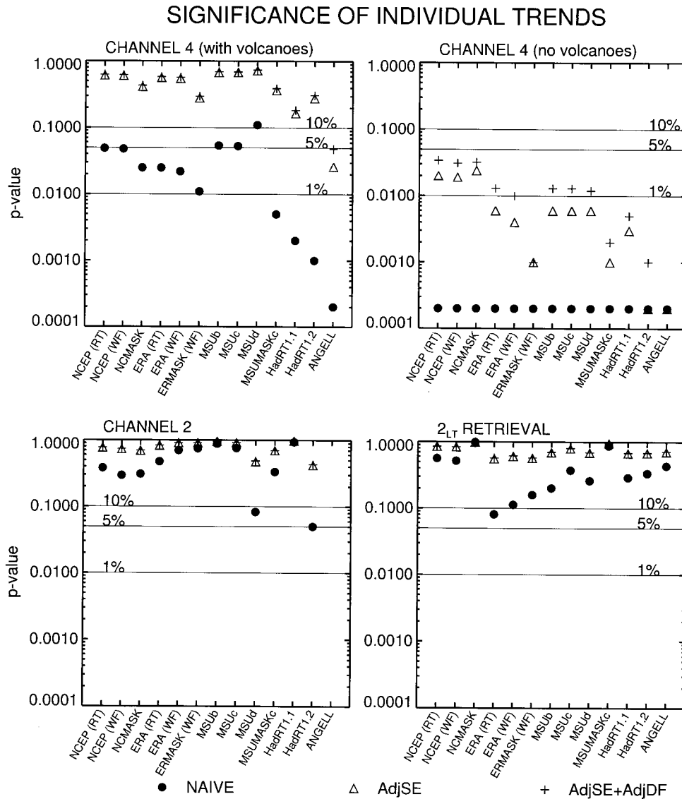
Figure 4. Significance of trends in individual time series of global-mean seasonal-mean temperature anomalies over 1979–1993. Results shown are p values for tests of the null hypothesis of zero trend, obtained using the NAIVE, AdjSE, and AdjSE + AdjDF approaches (see section 4.1). The nominal 1, 5, and 10% significance levels are indicated with thin horizontal lines. Note that for the channel 2 and 2_{LT} results, p values obtained with the AdjSE and AdjSE + AdjDF approaches are highly similar. In the case of channel 4 data that exclude volcanic effects, very small p values were set to 0.0002 to facilitate plotting.
