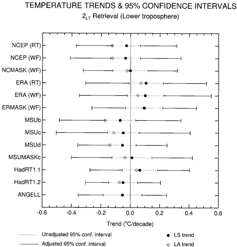
Figure 5. Unadjusted and adjusted 95% confidence intervals for least squares linear trends in lower tropospheric temperature ( 2_{LT} retrieval). All confidence intervals were computed with global-mean seasonal-mean anomaly data spanning the period 1979–1993. The smaller, unadjusted confidence intervals do not account for temporal autocorrelation and are estimated with the normal distribution. The adjusted 95% confidence intervals (shown here as extensions to the unadjusted intervals) account for temporal autocorrelation in the data and are estimated with the Student’s t distribution (see section 5.1). Trends computed with the LS and LA approaches are also shown.
