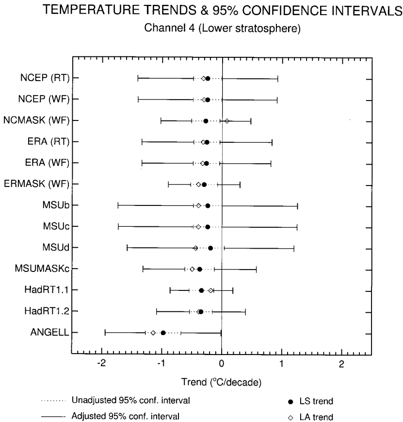
Figure 7. As for Figure 5, but for the lower stratosphere (channel 4).
