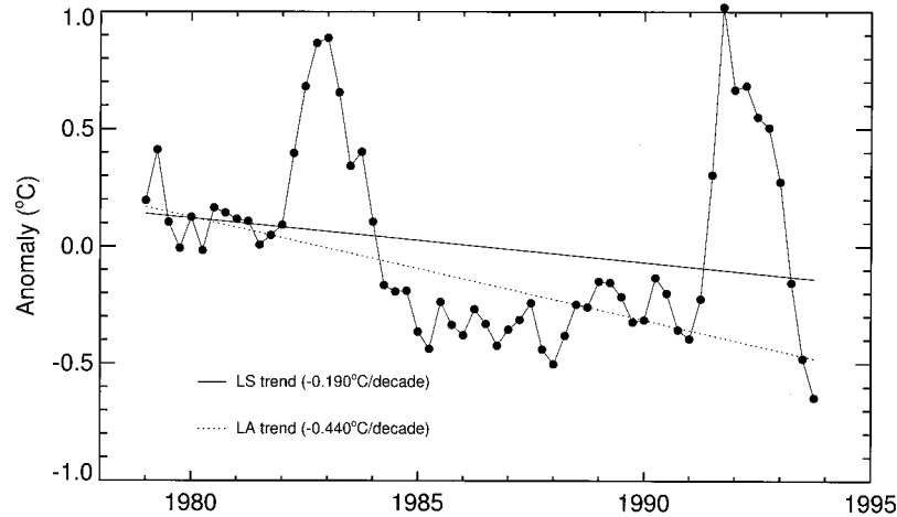
Figure 2. Time series of seasonal-mean lower stratospheric (channel 4) temperature anomalies ( ^{\circ}\text{C} ) over 1979–1993 in MSUd. Also shown are linear fits to the data using two approaches: least-squares (LS) and least-absolute deviations (LA).
