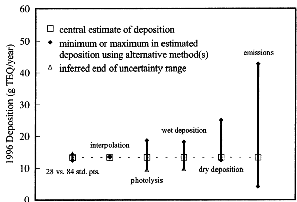
FIGURE 16. Uncertainties in model estimates of total 1996 dioxin deposition to Lake Superior. When variations in only one direction were evaluated, the other endpoint of the uncertainty range was inferred by assuming that the influence of the variation was approximately the same on either side of the central estimate.
