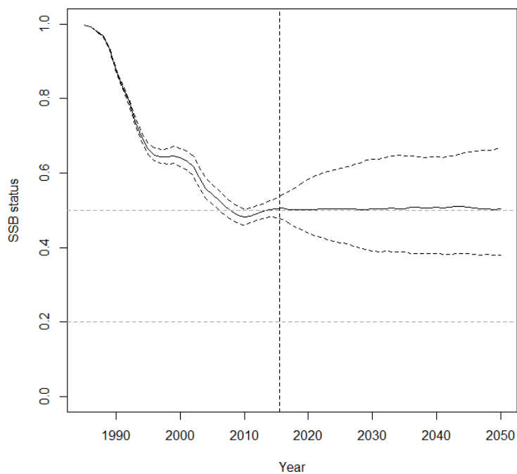
Figure A5: Dissostichus eginoides in Subarea 48.3: projection of SSB relative to virgin biomass for 35 years based on a constant catch of 2 750 tonnes per year. Confidence intervals at 10% and 90% shown as dashed lines. Vertical dashed line indicates the split between model fit to past data and projection. Horizontal lines indicate 50% and 20%
