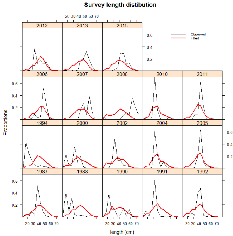
Figure A4: Dissostichus eginoides in Subarea 48.3: Observed length distributions (black) and model fits (red) to survey data.
