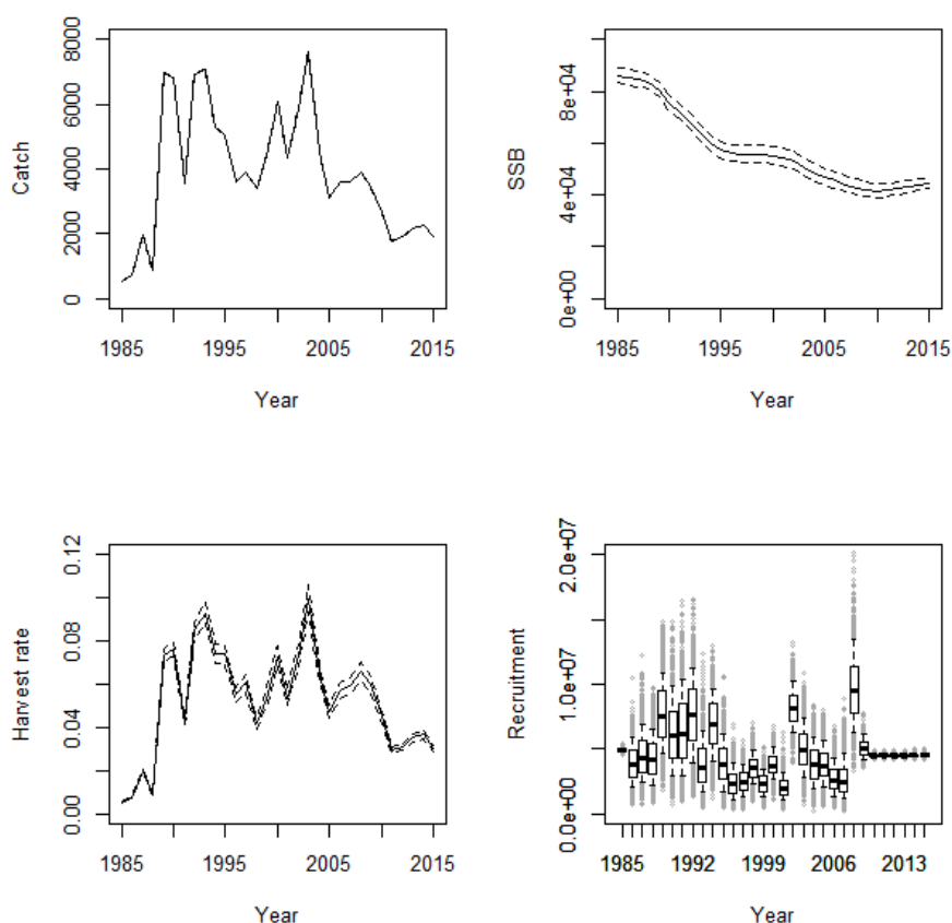
Figure A1: Dissostichus eleginoides in Subarea 48.3: Time series of catch, SSB, harvest rate and recruitment, with uncertainty estimated from MCMC resampling. Solid lines indicate the median value, dotted lines indicate the 10th and 90th percentiles and boxes extend from 25th to 75th percentiles.
