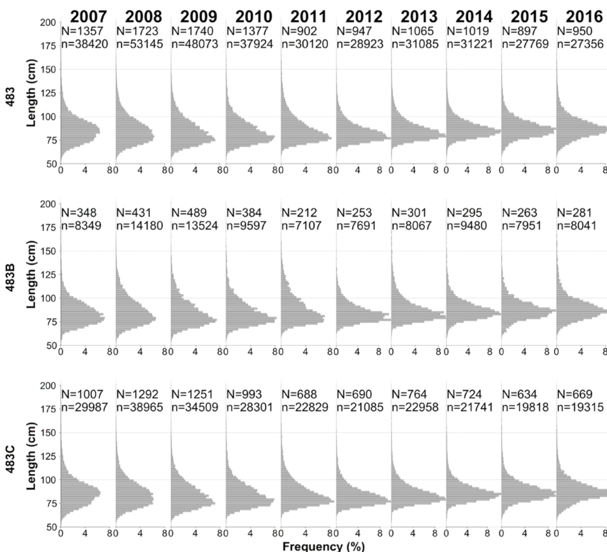
Figure 2: Length frequencies for Dissostichus eleginoides in Subarea 48.3 from 2007 to 2016 using observer data. The number of hauls (N) and the number of fish measured (n) in each year are given at the top of each panel. Letters to the left of the panel (B and C) refer to the management areas shown in Figure 1.
