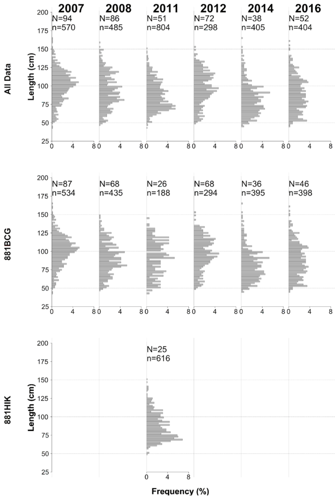
Figure 4: Annual length-frequency distributions of Dissostichus eginoides caught in Subarea 88.1 (top panel) and in each SSRU (lower panels). The number of hauls from which fish were measured (N) and the number of fish measured (n) in each year are provided.
