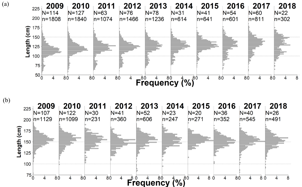
Figure 1: Annual length-frequency distributions for: (a) Dissostichus eleginoides , and (b) D. mawsoni in Subarea 48.4. The number of hauls from which fish were measured (N) and the number of fish measured (n) in each year are provided.
