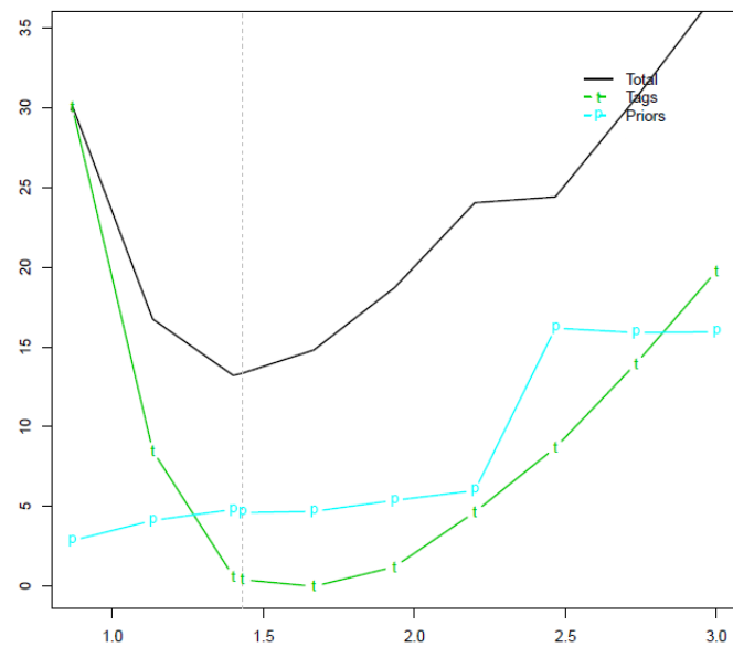
Figure A1: Dissostichus eleginoides in Subarea 48.4: Likelihood profiles for values of B_0 . Negative log likelihood values have been rescaled to have minimum 0 for each dataset. Vertical line indicates the overall MPD estimate of B_0 .
