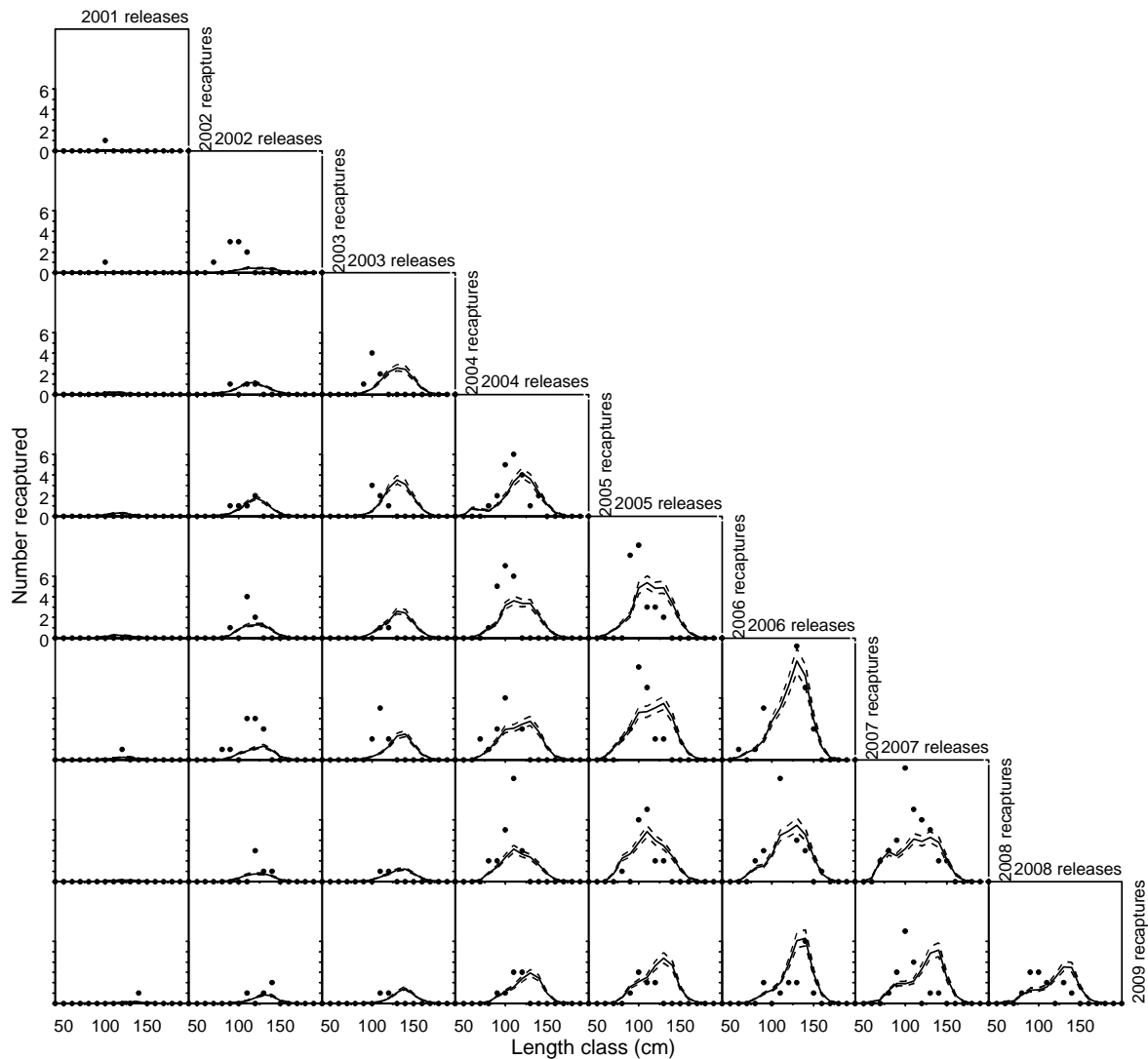
Figure 9: Observed (points) and posterior estimates (lines, MCMC median and 95% CI) of the number of tags recaptured (y-axis) by length class (x-axis), year of release (columns) and year of recapture (rows) for the Ross Sea base-case model.
