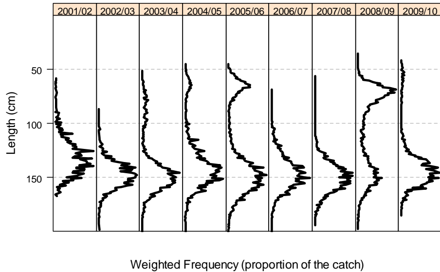
Figure 3: Catch-weighted length frequencies for Dissostichus mawsoni in Subarea 88.2 (source: observer, fine-scale and STATLANT data, and the length-weight relationship was taken from observations on D. mawsoni in Subarea 88.1).
