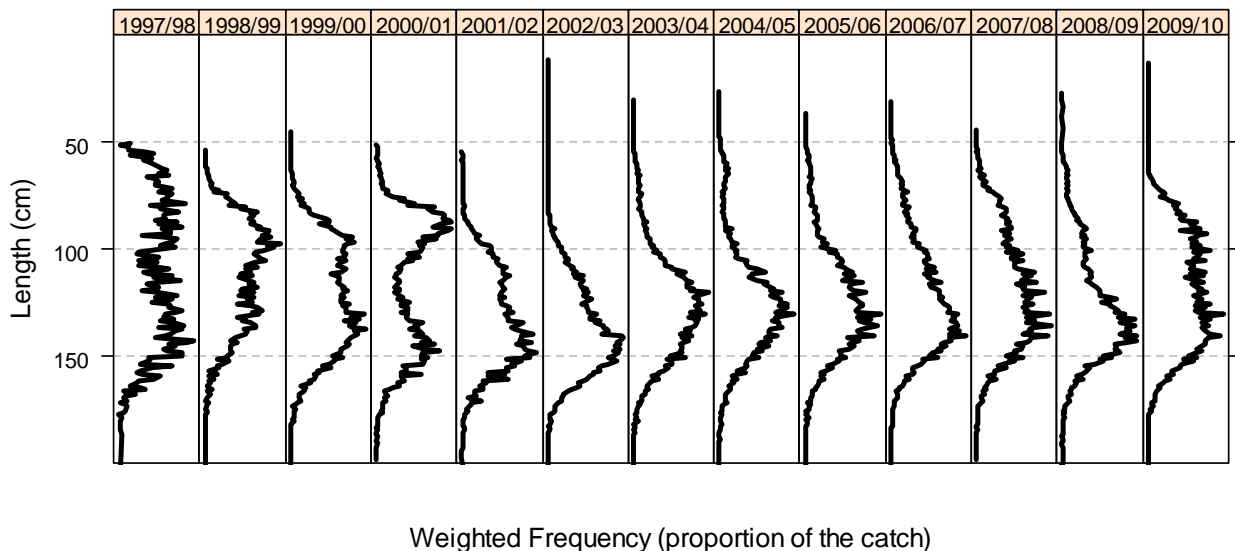
Figure 2: Catch-weighted length frequencies for Dissostichus mawsoni in Subarea 88.1 (source: observer, fine-scale and STATLANT data).
