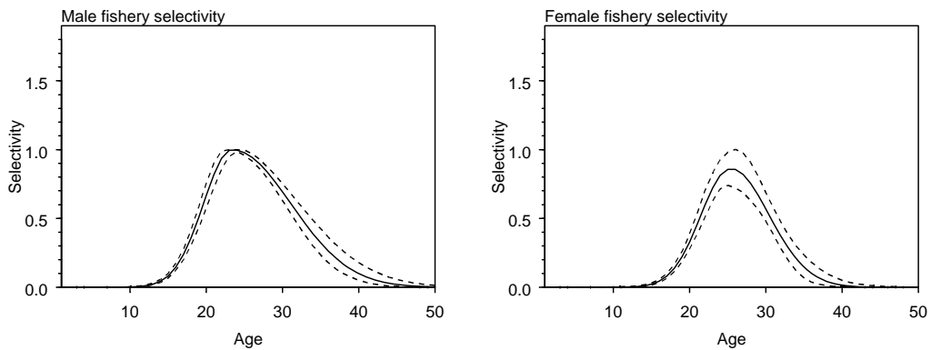
Figure 8: Estimated male and female selectivity ogives for the SSRU 882E base-case model (solid lines indicate the median, and dashed lines indicate the marginal 95% CI).
