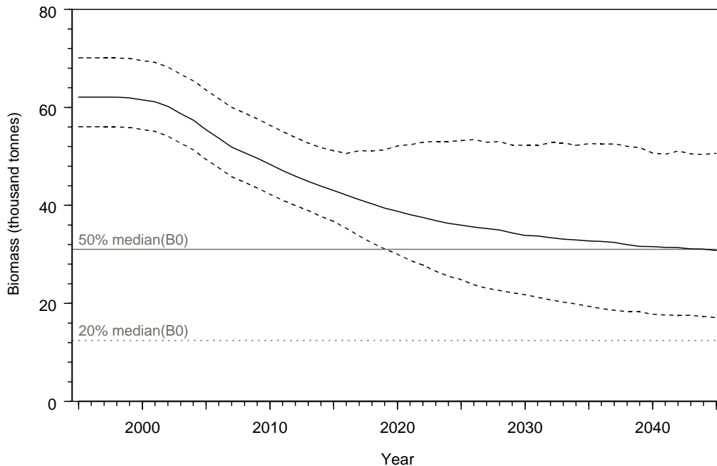
Figure 5: Estimated spawning stock biomass median (solid line) and 95% CI (dashed lines) for the base-case Ross Sea model.
