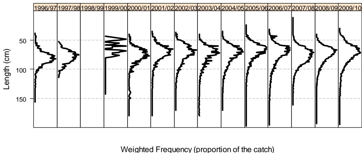
Figure 2: Catch-weighted length frequencies for Dissostichus eleginoides caught by longline in the French EEZ in Subarea 58.6 (source: fine-scale and STATLANT data, and the length–weight relationship was taken from observations on D. eleginoides in Subarea 58.7).
