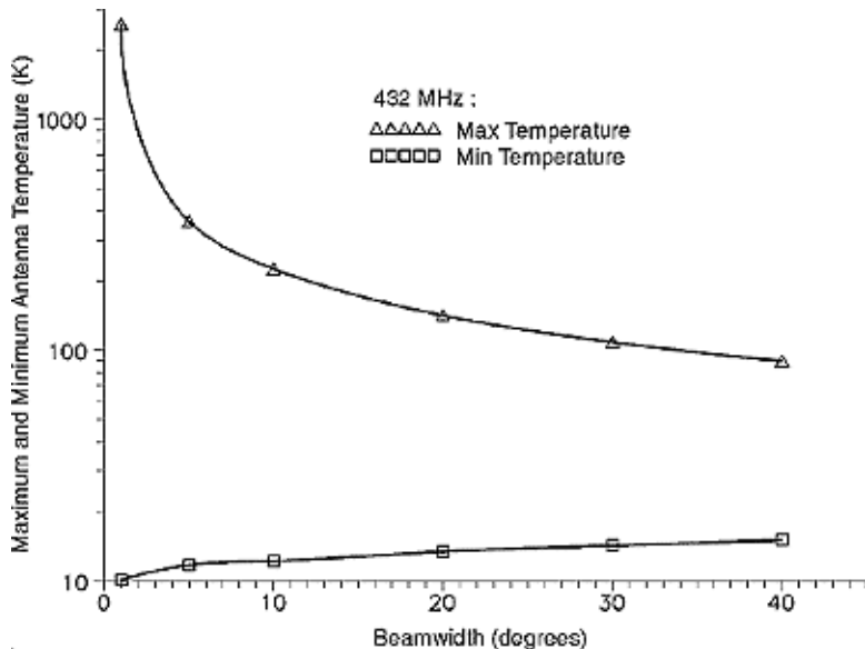
Figure 3—The effect of antenna beamwidth on the expected antenna temperatures, that we might observe at 432 MHz. Note the logarithmic intensity scale. While the minimum sky temperature changes relatively little, from 15 K with a 40° beam down to 10 K with a 1° beam, the peak temperatures vary from ~90 K (40° beam) up to ~2500 K (1° beam). For all but the smallest beam size, the galactic nucleus gives the highest antenna temperature. With an angular resolution of 1° or better, the discrete source Cassiopeia A becomes the brightest point in the radio sky at this wavelength.
