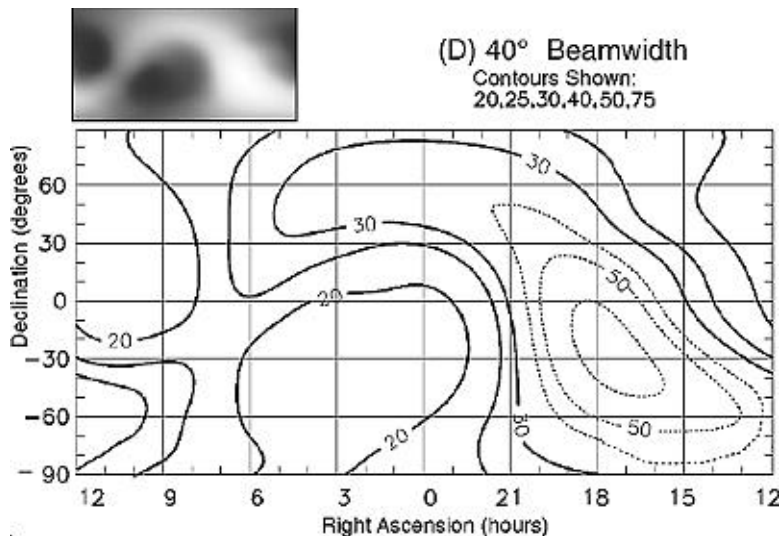
Figure 2 —Gray-scale images and contour plots show the expected sky brightness temperature at 432 MHz, for beamwidths from 5 to 40°. Contours of 40 K and greater are drawn as dashed lines. Contours show the level of sky noise collected by an antenna pointing in any specific direction. As with Figure 1, the coordinates are RA,dec (epoch B1950), with RA = 0 h, dec = 0° at the center. Sagittarius A, the galactic nucleus at RA = 17.8 h, dec = -28.9° (epoch J2000), is the strongest source of emission in each plot.
