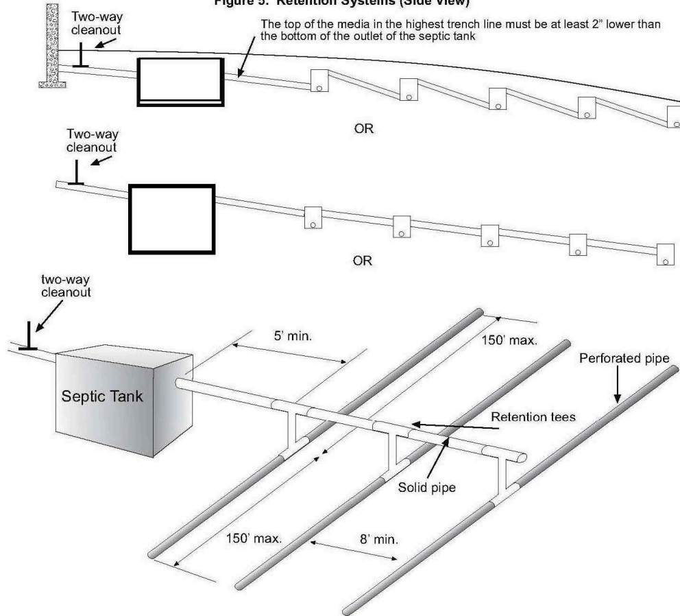
Figure 5. Retention Systems (Side View)
