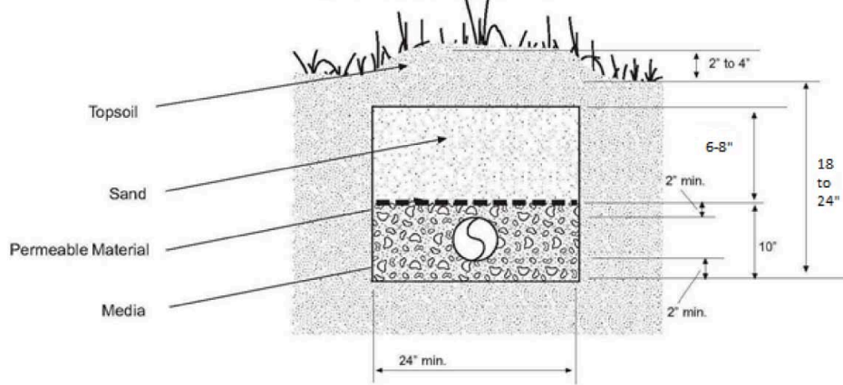
Figure 3. Cross-Section of Low Pressure Dosing
