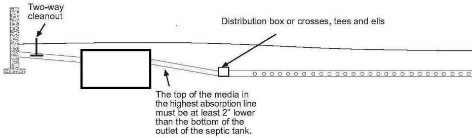
Figure 2. Level Systems (Side View)
